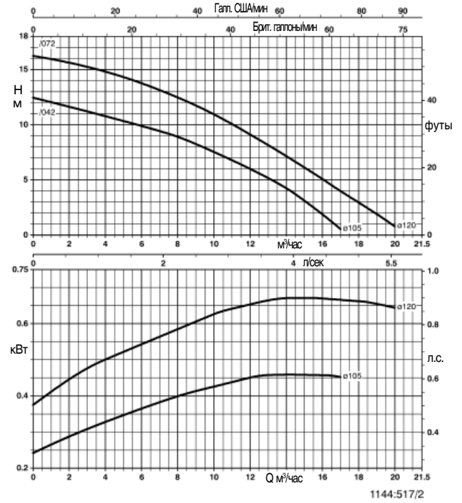
Trialine Z 32-125
