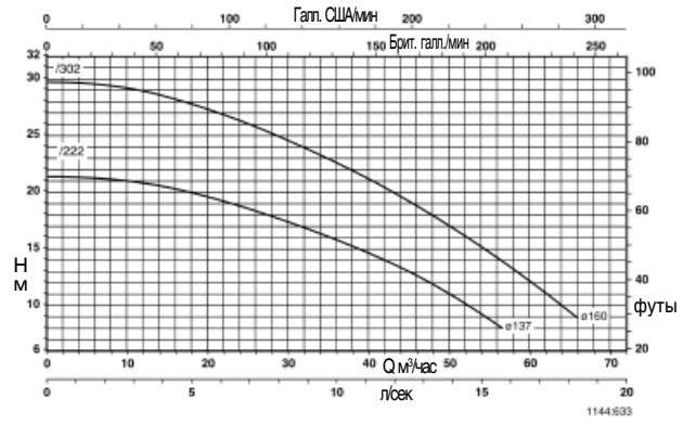
Trialine Z 40-160
