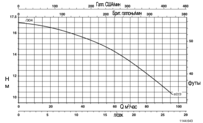
Trialine Z 65-250
