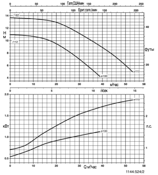
Trialine Z 65-125
