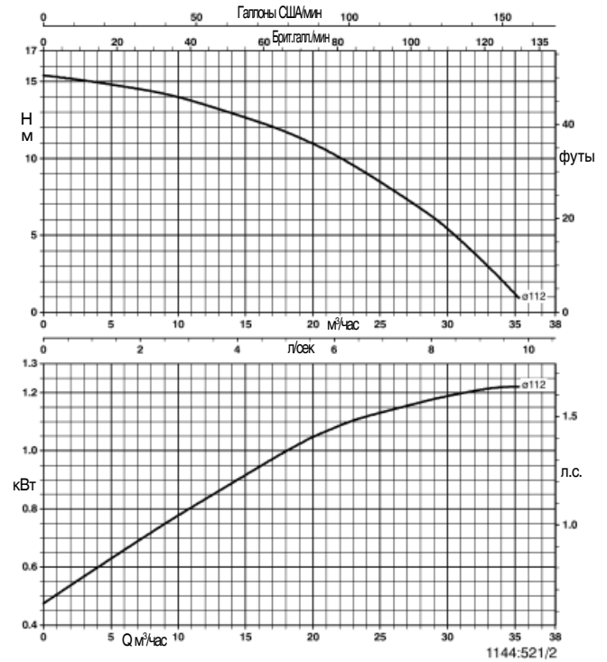
Trialine Z 40-125/132
