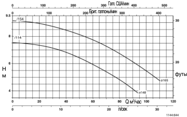
Trialine Z 80-160
