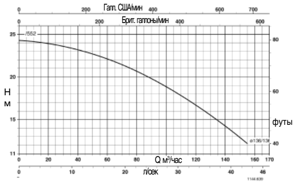
Trialine Z 32-160
