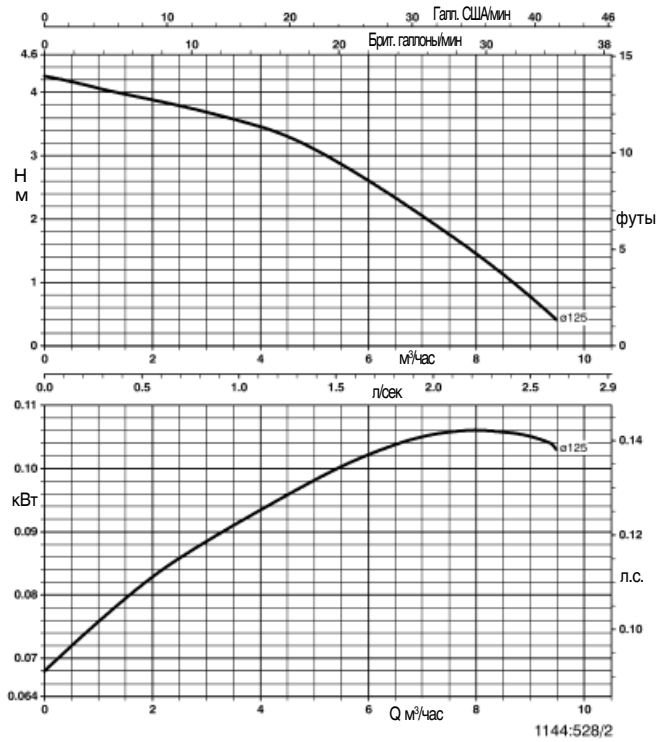
Trialine Z 32-125/014
