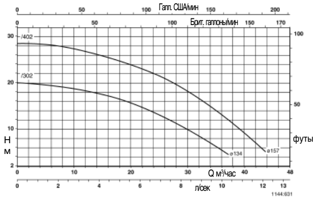
Trialine Z 32-160
